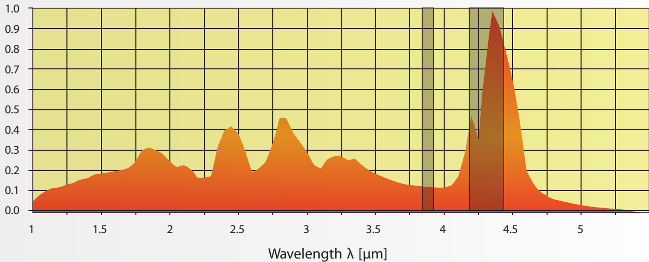
Figure 9. Flame absorption spectrum of a gas-fired furnace with two types for filters for different measurement applications
