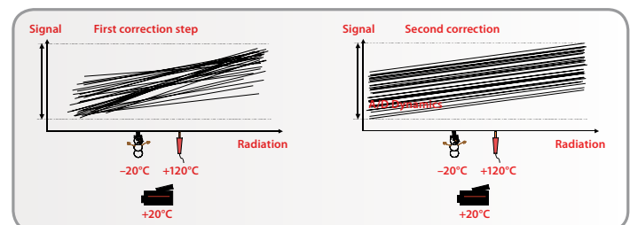
Figure 10. After offset compensation, slope correction is applied.
