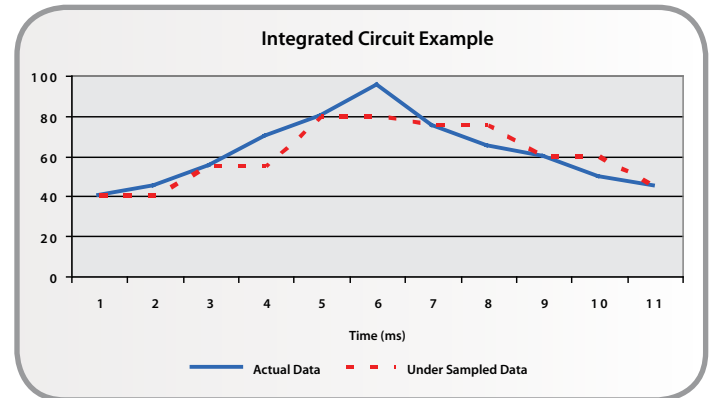
Figure 3. Maximum IC temperature data – actual vs. undersampled
