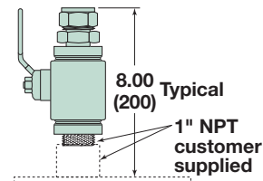
Valve with Compression Fitting (089- 5218-001)
