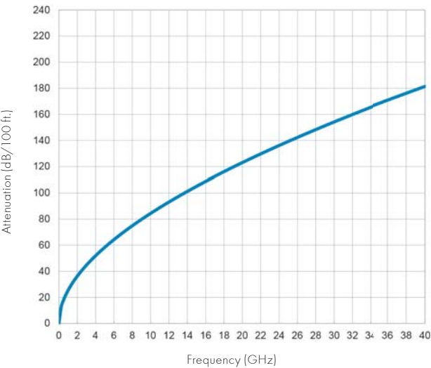
Graph 1: Cable attenuation
