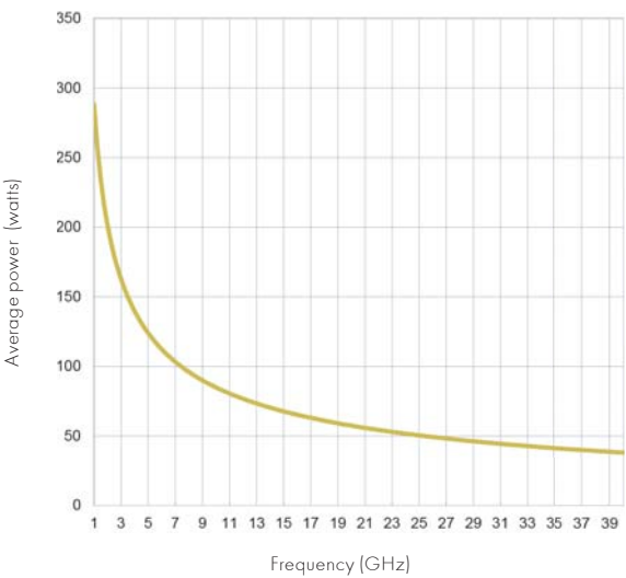
Graph 2: Max. power handling (25°C at sea level)
