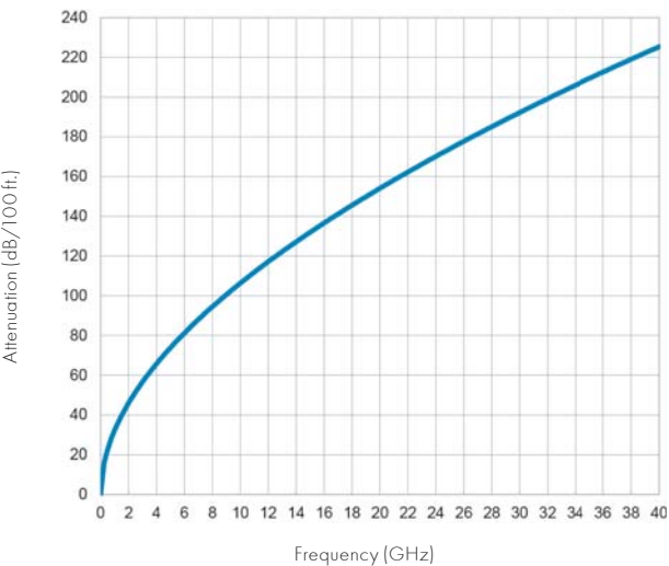
Graph 1: Cable attenuation
