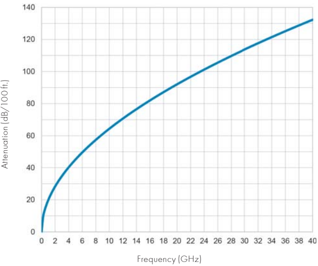
Graph 1: Cable attenuation
