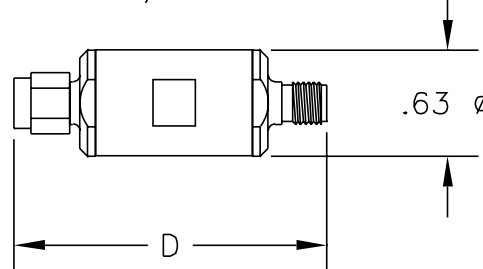
SMA MALE / SMA FEMALE
