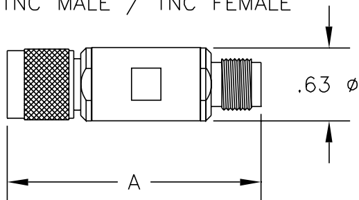
TNC MALE / TNC FEMALE
