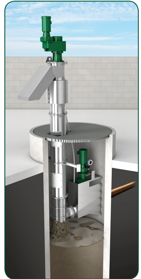
Wall mounted screening basket with spiral lifting screw and a patented compaction zone
