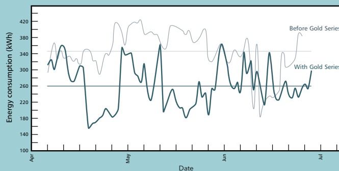
Energy consumption Before and after installation of Gold Series
