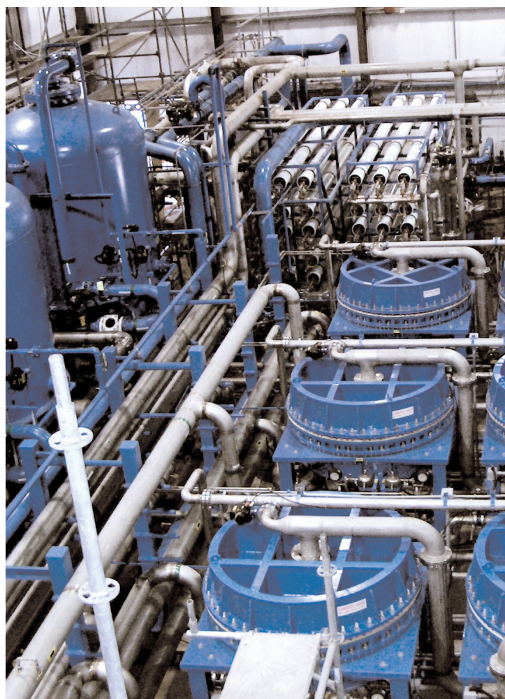
Two trains, peripherals and a remote monitoring station in a 70 ft X 120 ft space
