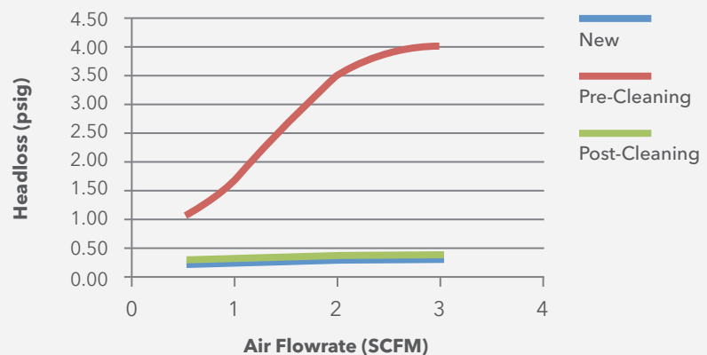
Effect of Diffuser Cleaning on Headloss at an MBR Plant with Ceramic Diffusers
