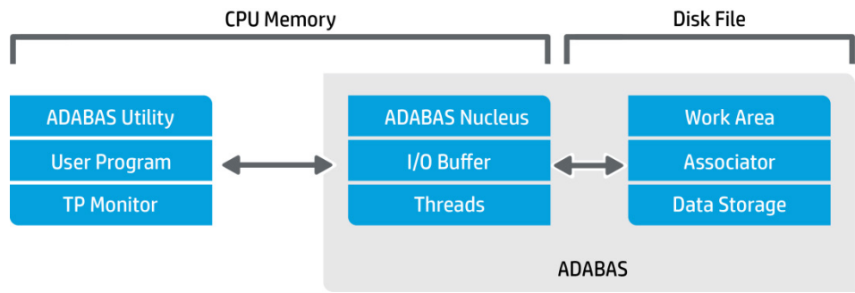
Figure 2. Entire network multi-system processing tool
