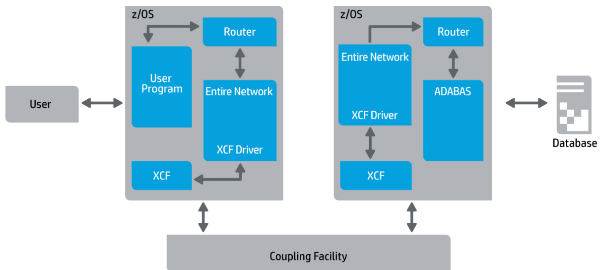
Figure 3. Cluster services with other ADABAS products (ADABAS online system communicates with all nucleuses within the Sysplex cluster)
